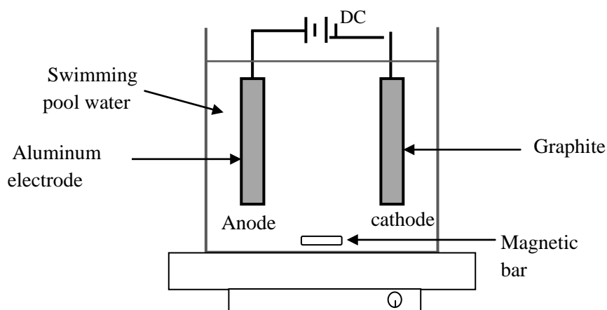
Figure 1. Electrocoagulation scheme.
